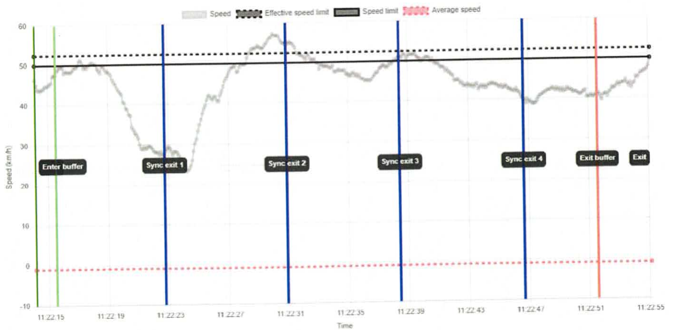
Speed graph over "SZ PS3-6 Montevaso" for "023"
